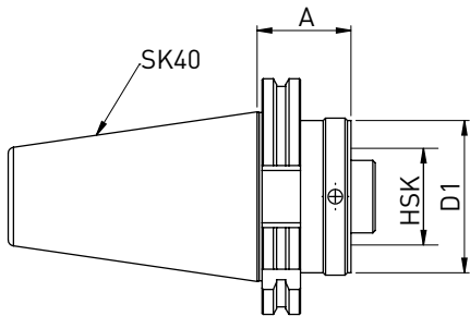
Adapter SK40 to HSK
