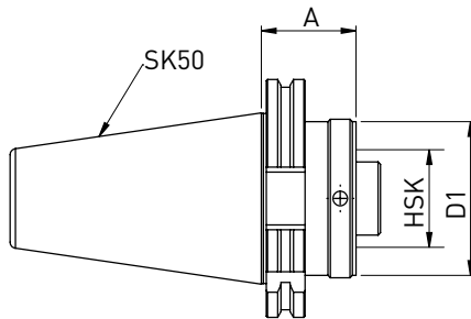
Adapter SK50 to HSK
