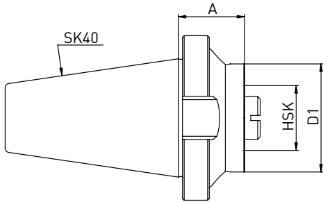
Adapter SK40 to HSK
