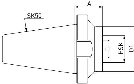
Adapter SK50 to HSK
