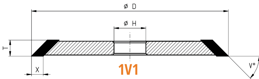
1V1 diamond wheels in stock
