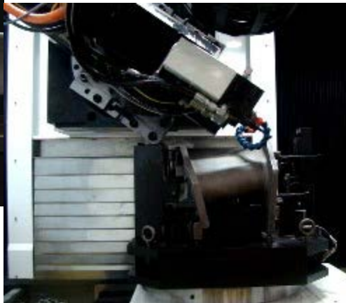
Vector Drilling
