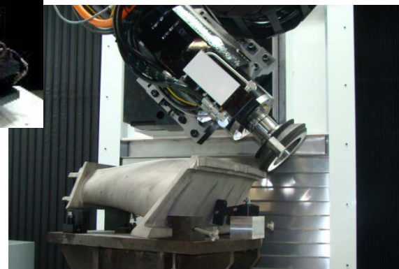
Grinding
