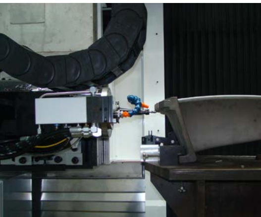
Milling
